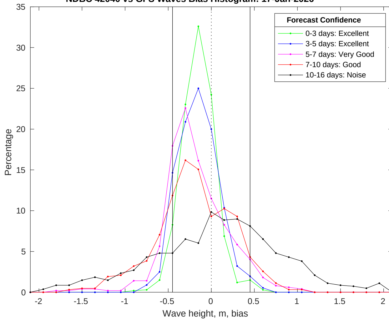
NDBC 42040 vs GFS Waves Bias Histogram: 17-Jan-2026
