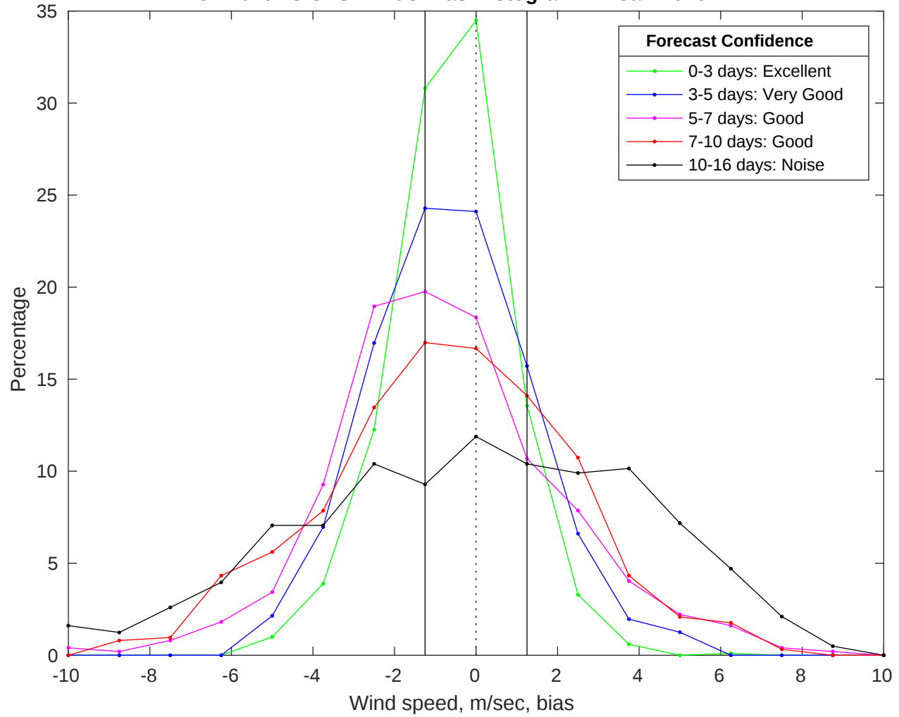
NDBC 42040 vs GFS Winds Bias Histogram: 17-Jan-2026
