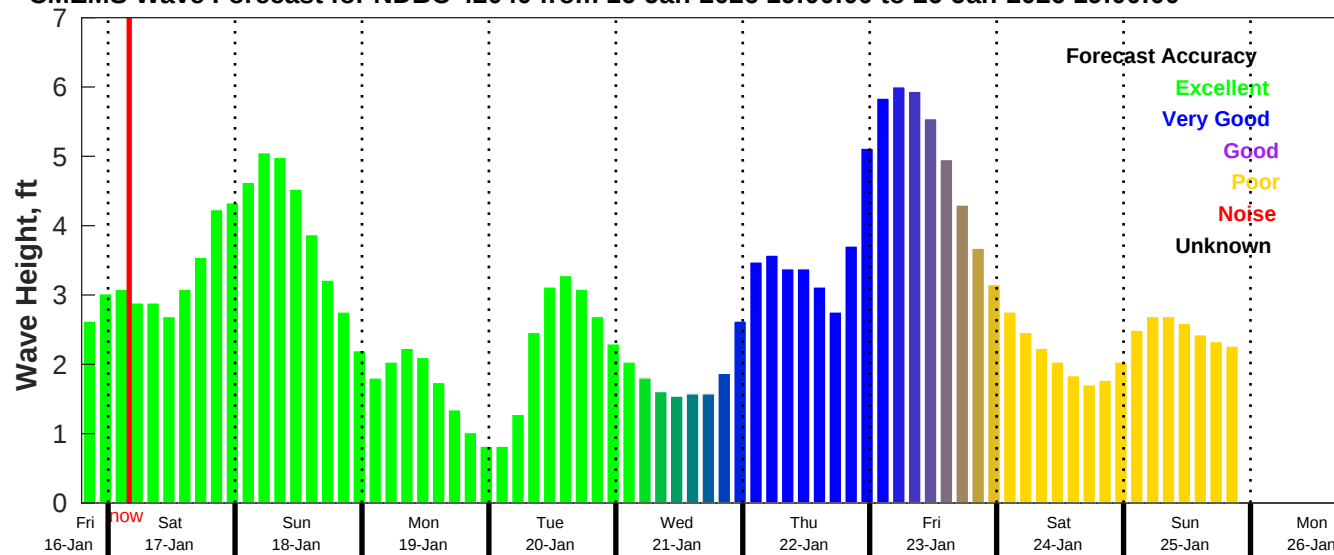
CMEMS Wave Forecast for NDBC 42040 from 16-Jan-2026 19:00:00 to 26-Jan-2026 19:00:00
