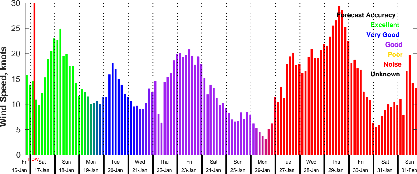
GFS Wind Speed Forecast for NDBC 42040 from 16-Jan-2026 19:00:00 to 01-Feb-2026 19:00:00
