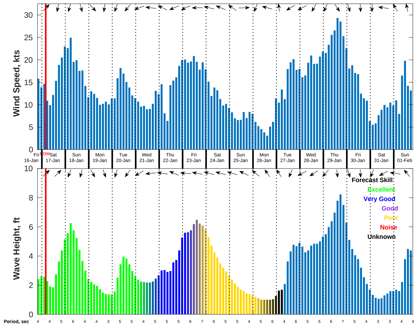
Wind & Wave Forecast for NDBC 42040 from 16-Jan-2026 19:00:00 to 01-Feb-2026 19:00:00
