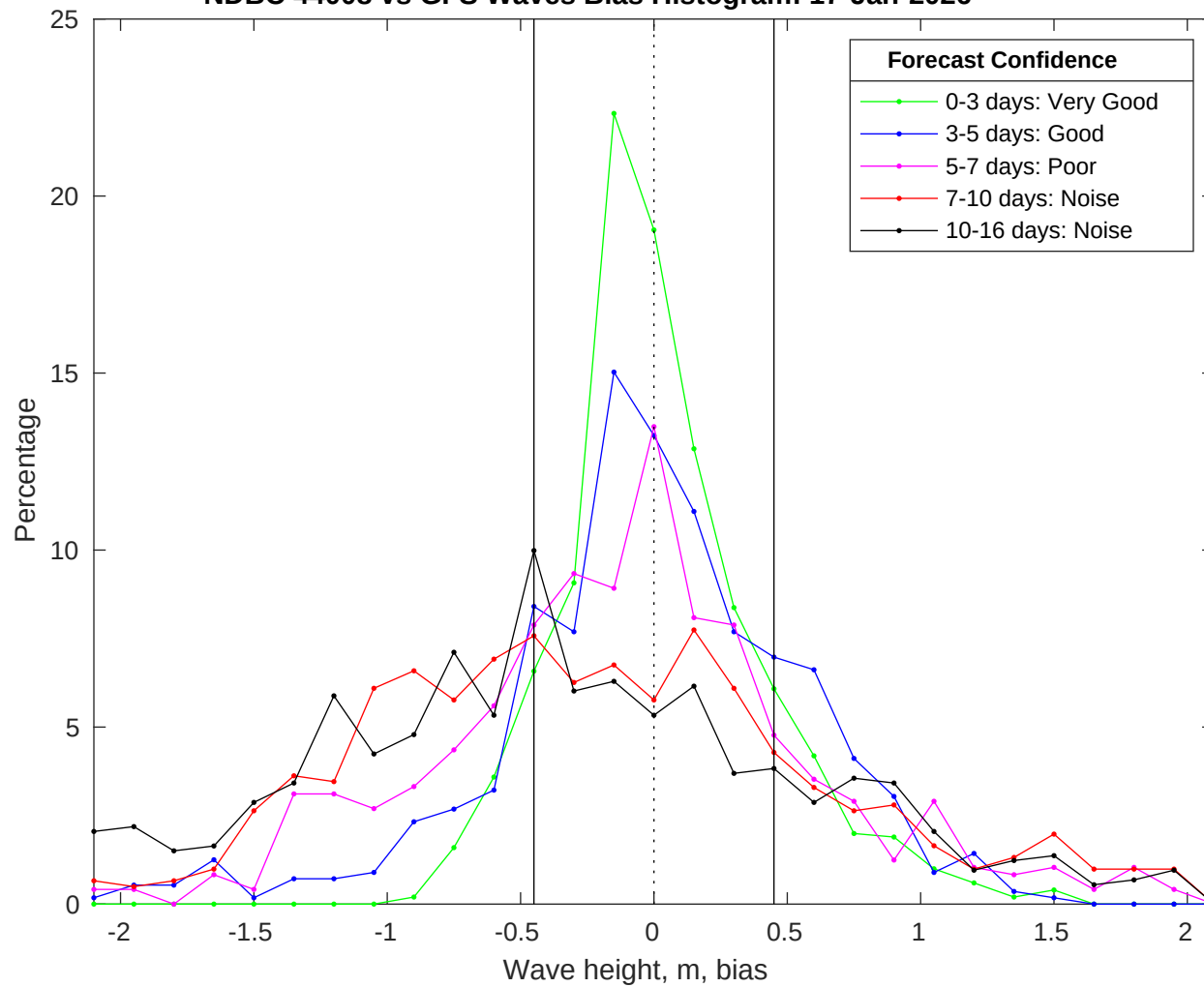
NDBC 44008 vs GFS Waves Bias Histogram: 17-Jan-2026
