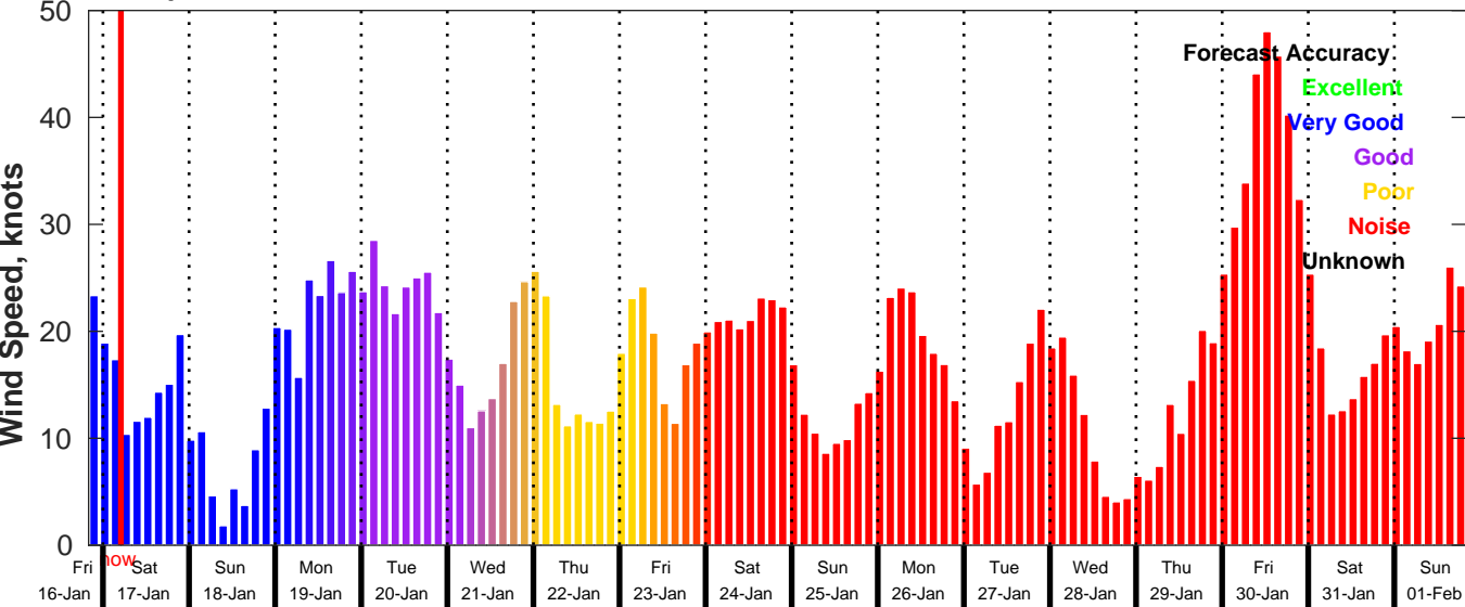
GFS Wind Speed Forecast for NDBC 44008 from 16-Jan-2026 20:00:00 to 01-Feb-2026 20:00:00
