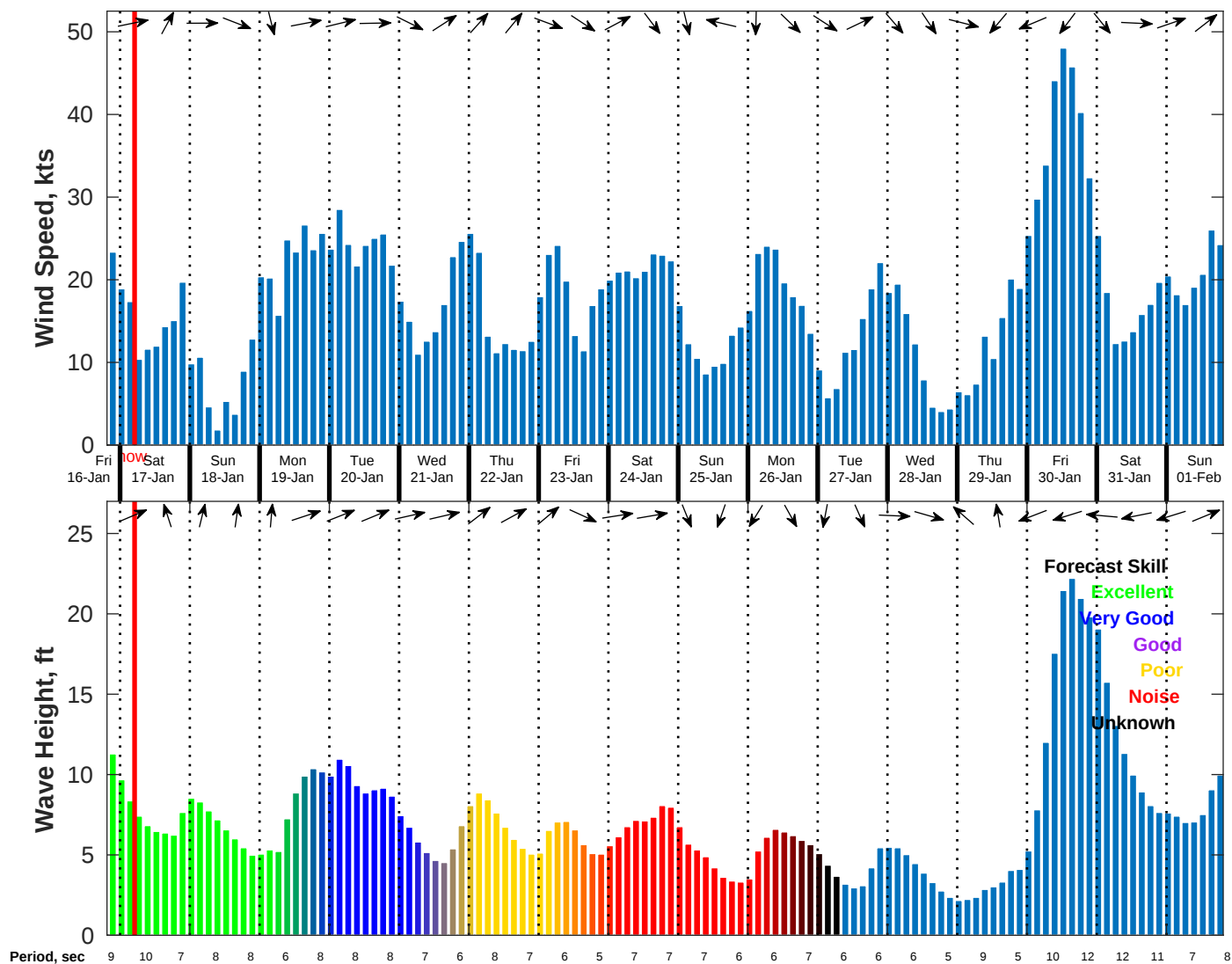
Wind & Wave Forecast for NDBC 44008 from 16-Jan-2026 20:00:00 to 01-Feb-2026 20:00:00
