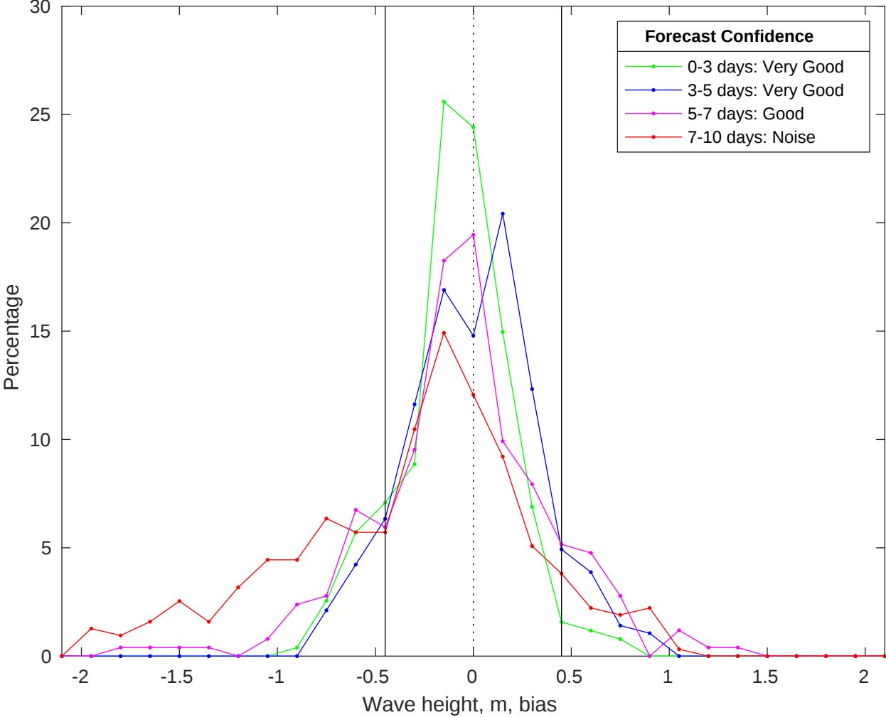
NDBC 46011 vs CMEMS Waves Bias Histogram: 17-Jan-2026
