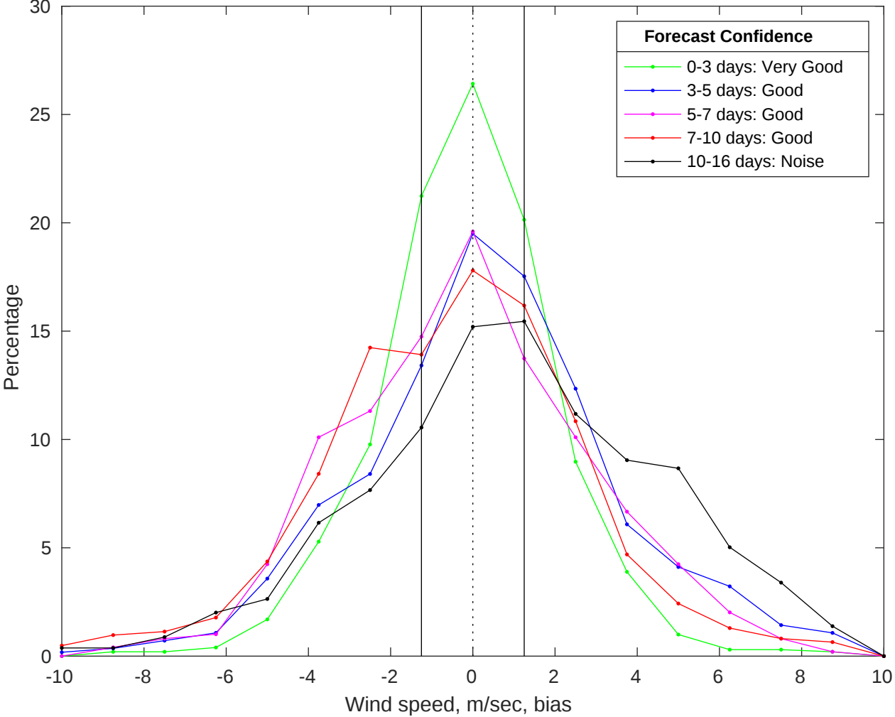
NDBC 46011 vs GFS Winds Bias Histogram: 17-Jan-2026
