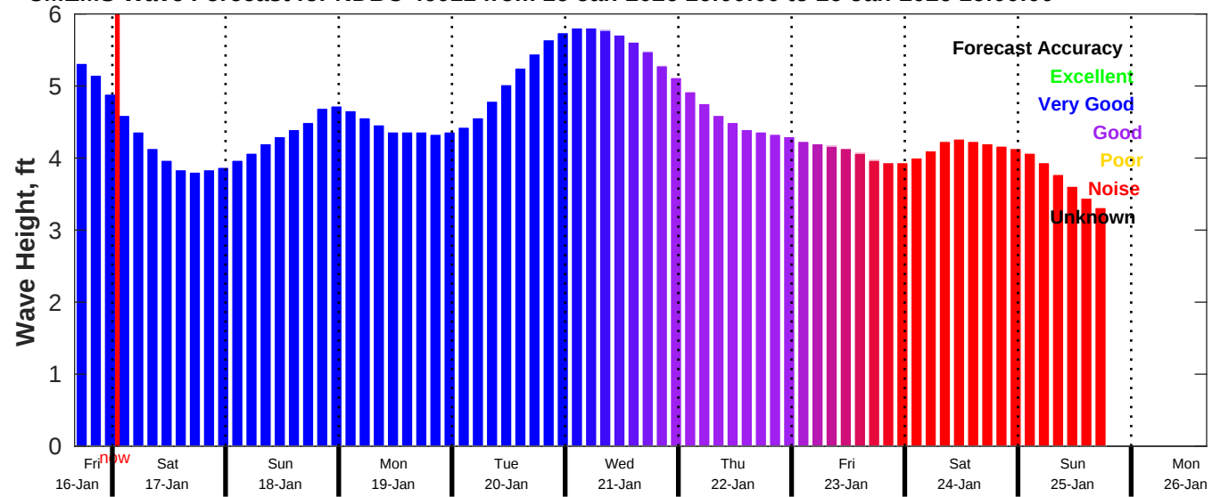
CMEMS Wave Forecast for NDBC 46011 from 16-Jan-2026 16:00:00 to 26-Jan-2026 16:00:00
