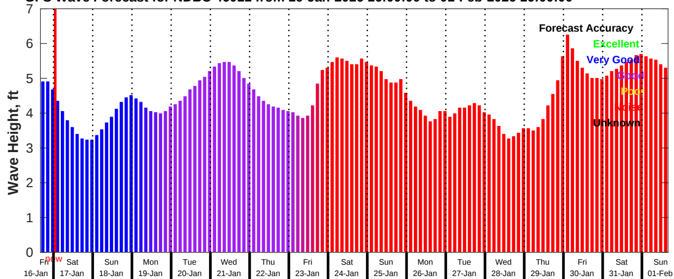
GFS Wave Forecast for NDBC 46011 from 16-Jan-2026 16:00:00 to 01-Feb-2026 16:00:00
