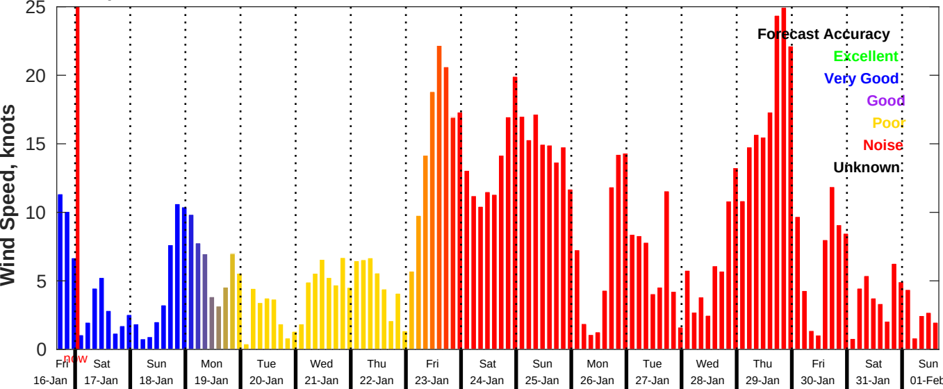
GFS Wind Speed Forecast for NDBC 46028 from 16-Jan-2026 16:00:00 to 01-Feb-2026 16:00:00
