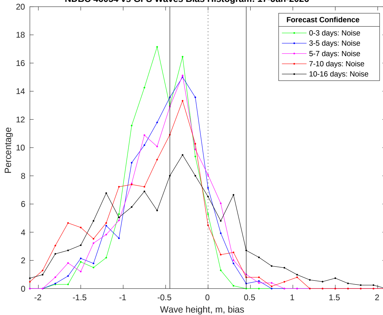
NDBC 46054 vs GFS Waves Bias Histogram: 17-Jan-2026
