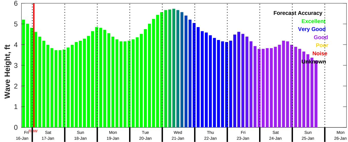
CMEMS Wave Forecast for NDBC 46054 from 16-Jan-2026 16:00:00 to 26-Jan-2026 16:00:00
