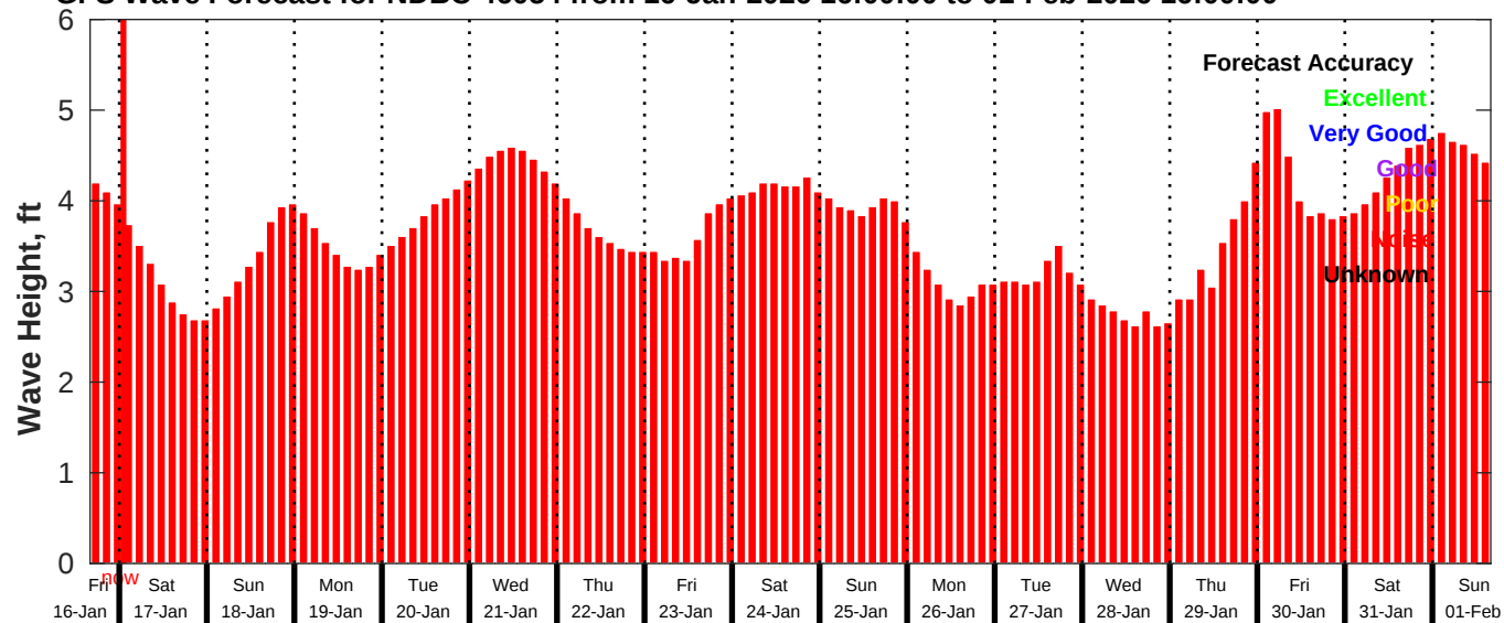
GFS Wave Forecast for NDBC 46054 from 16-Jan-2026 16:00:00 to 01-Feb-2026 16:00:00
