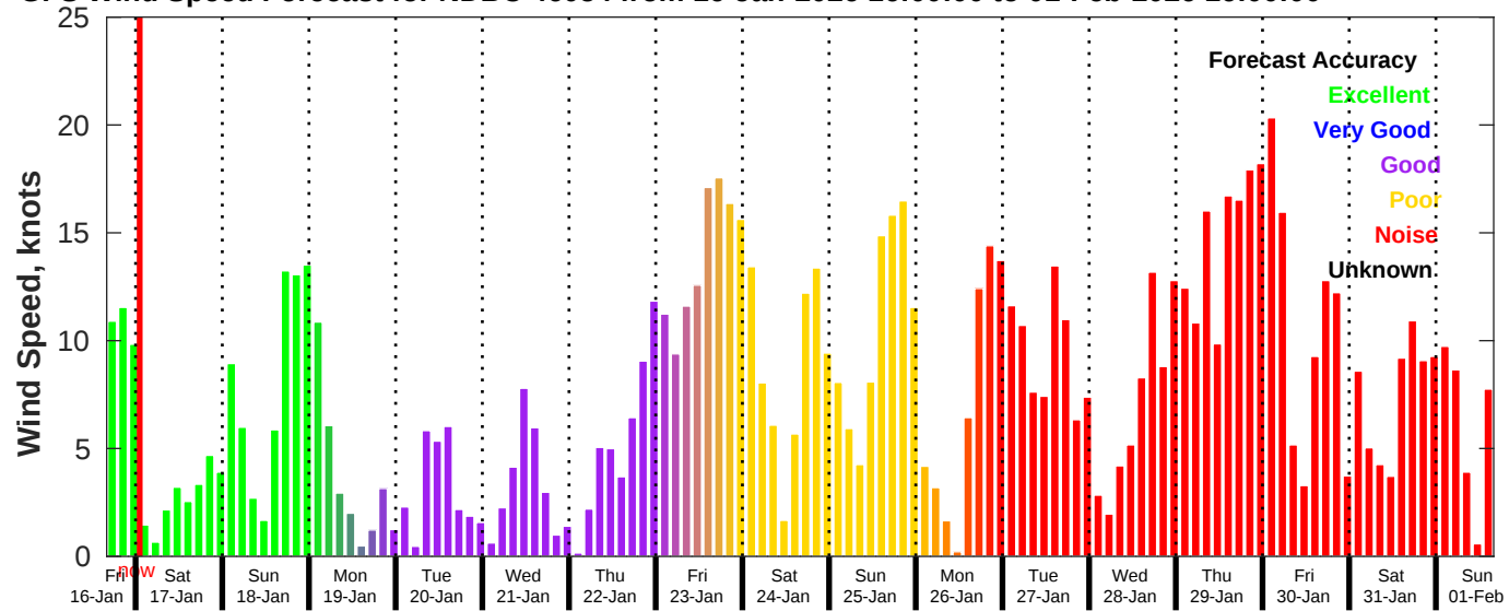
GFS Wind Speed Forecast for NDBC 46054 from 16-Jan-2026 16:00:00 to 01-Feb-2026 16:00:00
