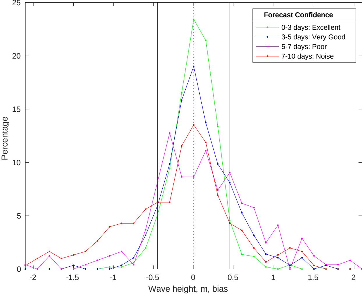
NDBC 46059 vs CMEMS Waves Bias Histogram: 17-Jan-2026
