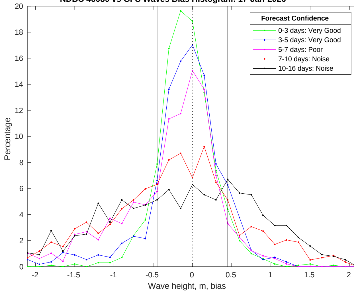
NDBC 46059 vs GFS Waves Bias Histogram: 17-Jan-2026
