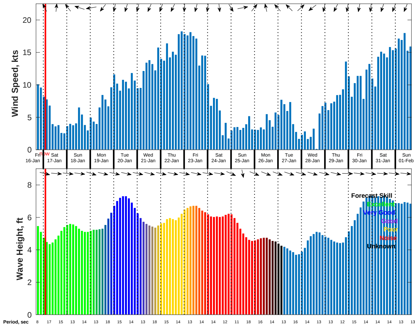
Wind & Wave Forecast for NDBC 46059 from 16-Jan-2026 17:00:00 to 01-Feb-2026 17:00:00
