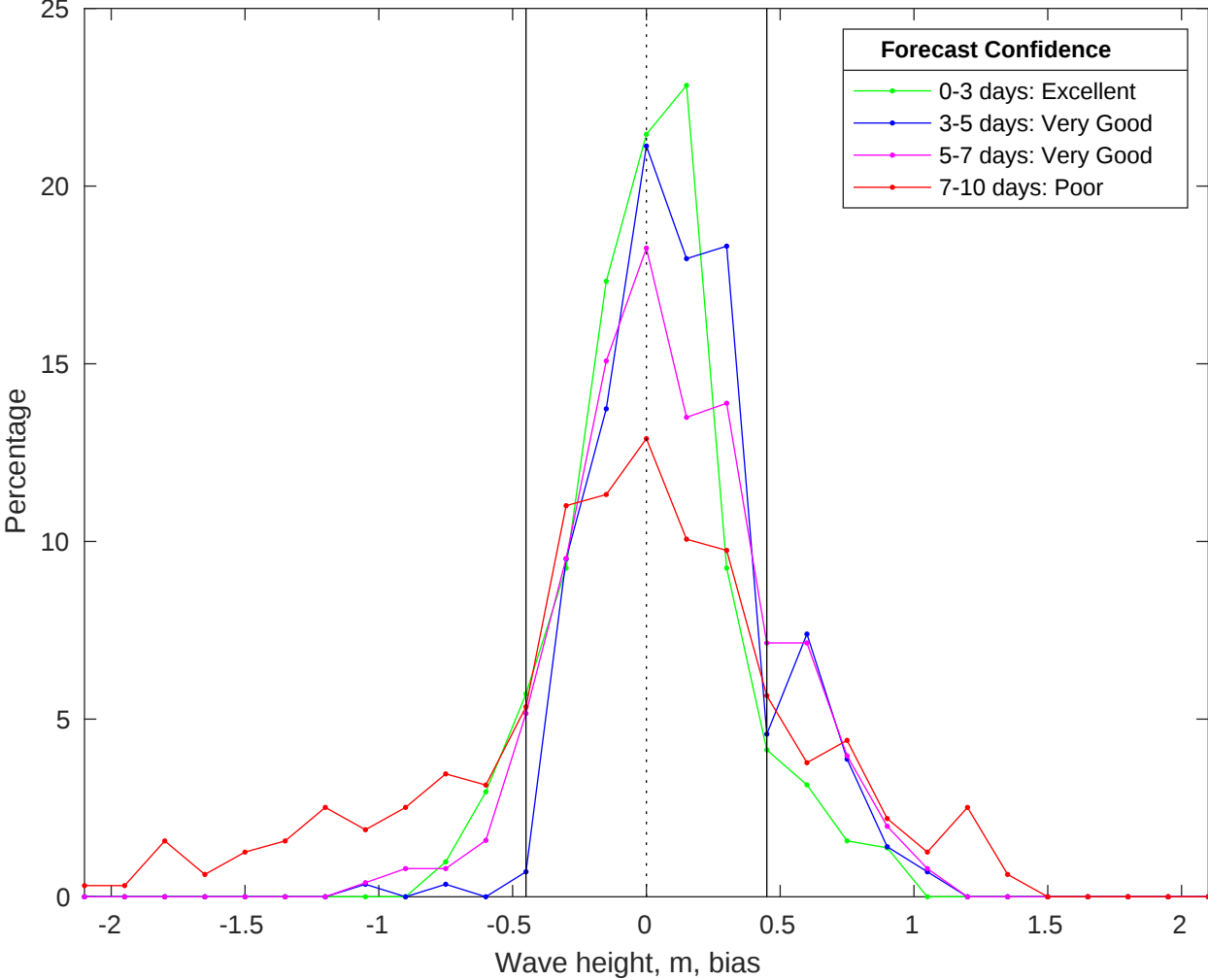
NDBC 46069 vs CMEMS Waves Bias Histogram: 17-Jan-2026
