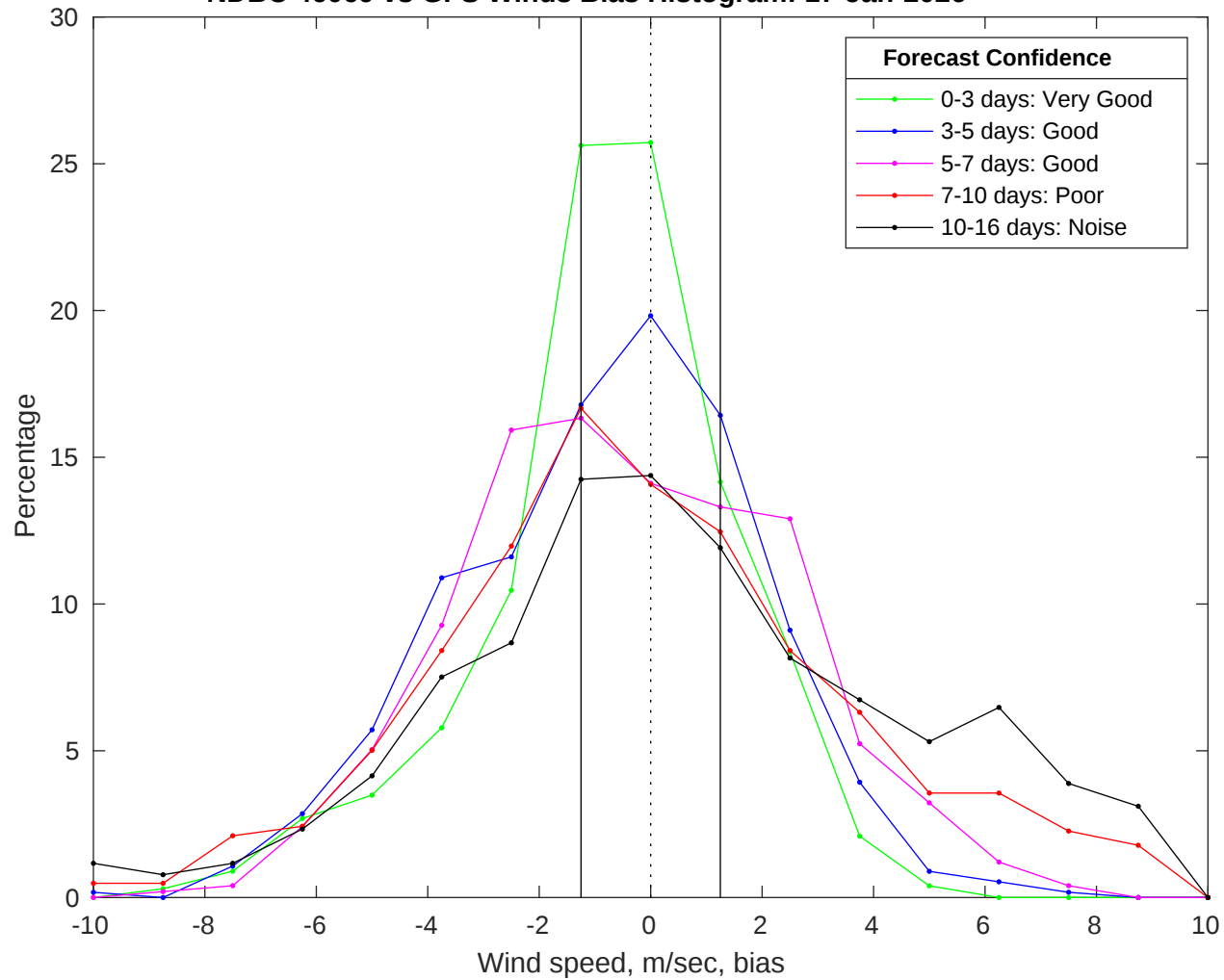
NDBC 46069 vs GFS Winds Bias Histogram: 17-Jan-2026
