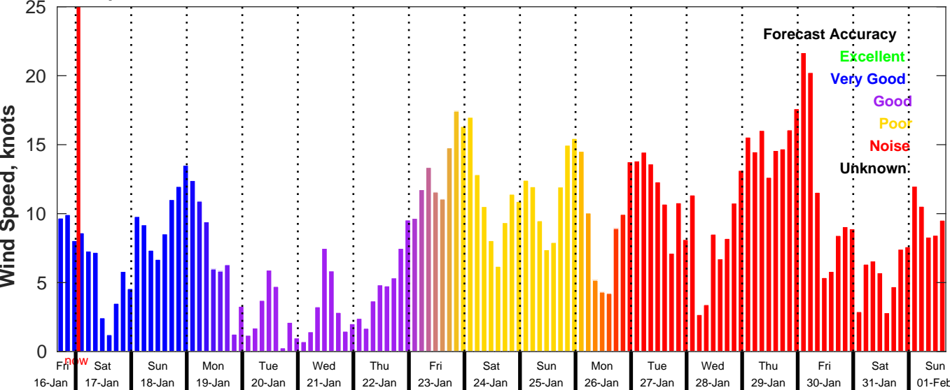
GFS Wind Speed Forecast for NDBC 46069 from 16-Jan-2026 16:00:00 to 01-Feb-2026 16:00:00
