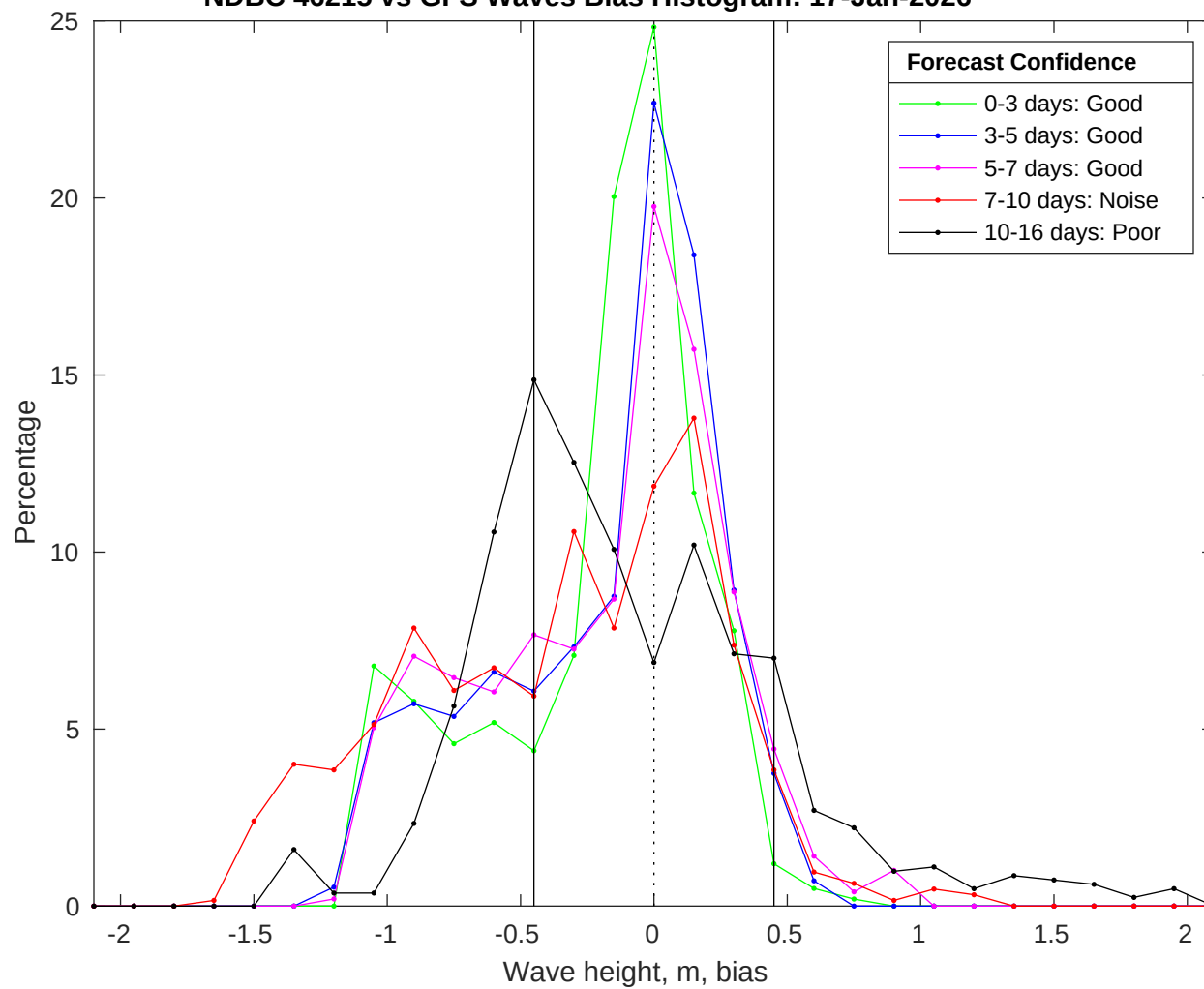
NDBC 46215 vs GFS Waves Bias Histogram: 17-Jan-2026
