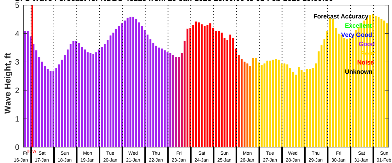
GFS Wave Forecast for NDBC 46215 from 16-Jan-2026 16:00:00 to 01-Feb-2026 16:00:00
