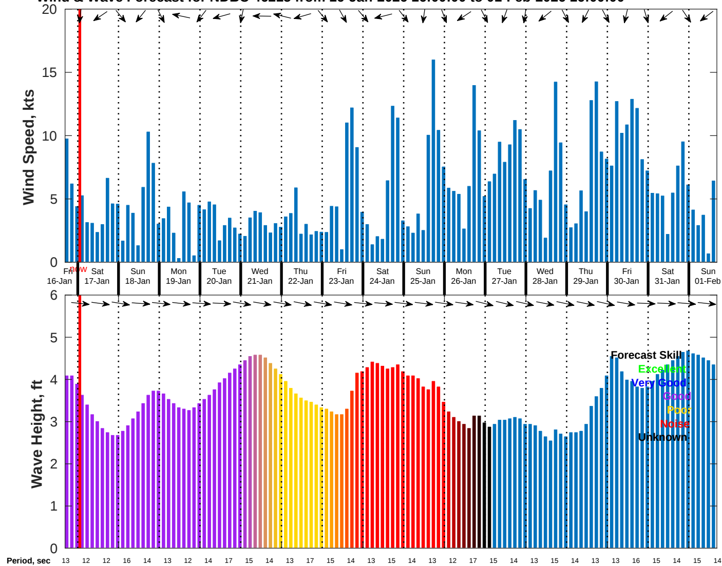
Wind & Wave Forecast for NDBC 46215 from 16-Jan-2026 16:00:00 to 01-Feb-2026 16:00:00
