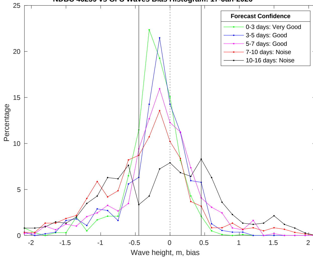
NDBC 46259 vs GFS Waves Bias Histogram: 17-Jan-2026
