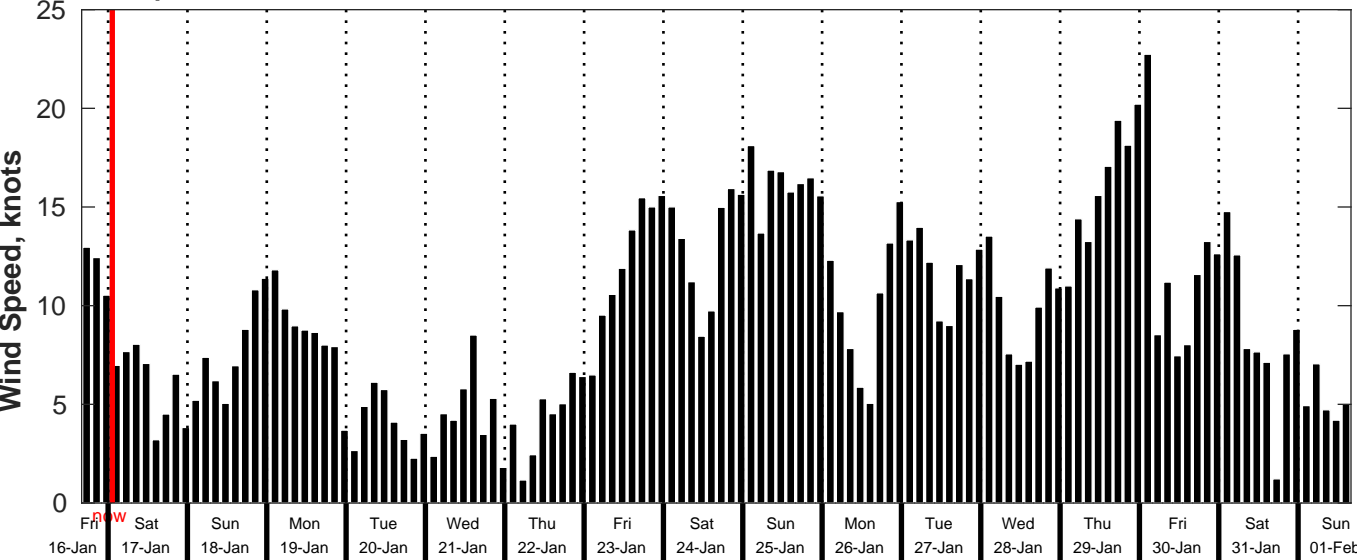
GFS Wind Speed Forecast for NDBC 46259 from 16-Jan-2026 16:00:00 to 01-Feb-2026 16:00:00
