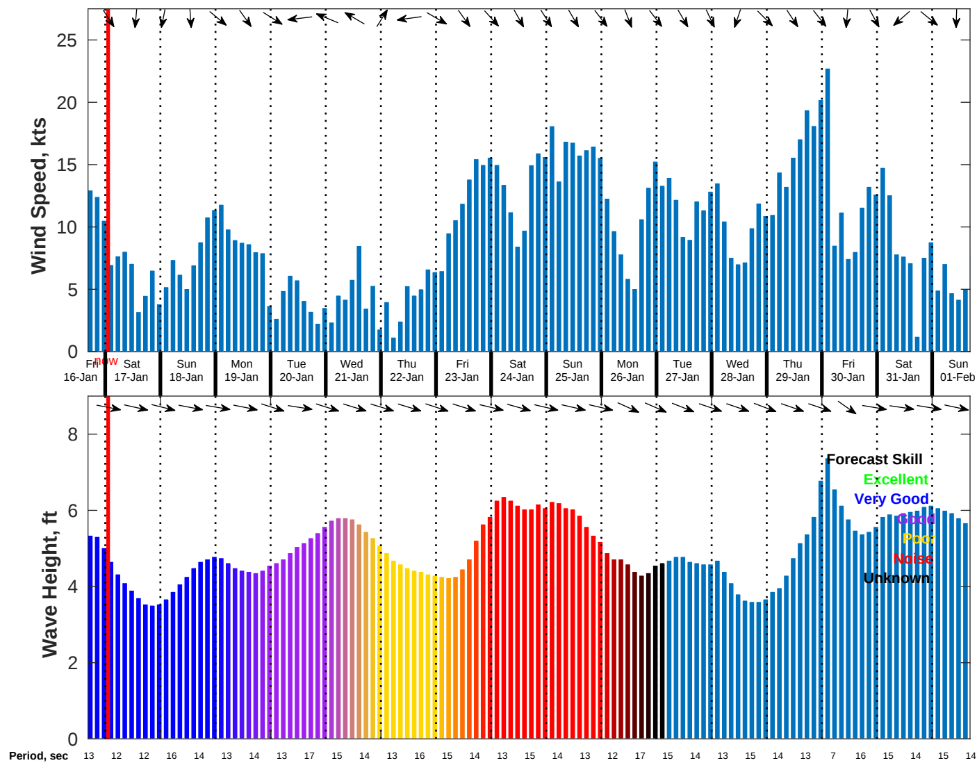
Wind & Wave Forecast for NDBC 46259 from 16-Jan-2026 16:00:00 to 01-Feb-2026 16:00:00
