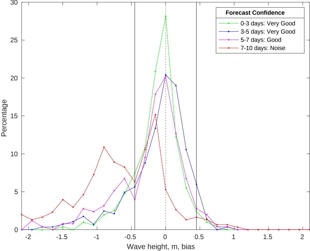
NDBC 51000 vs CMEMS Waves Bias Histogram: 17-Jan-2026
