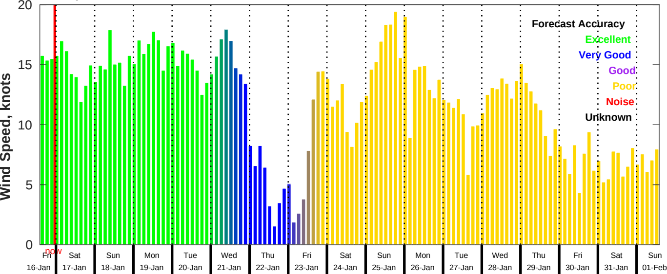
GFS Wind Speed Forecast for NDBC 51000 from 16-Jan-2026 14:00:00 to 01-Feb-2026 14:00:00
