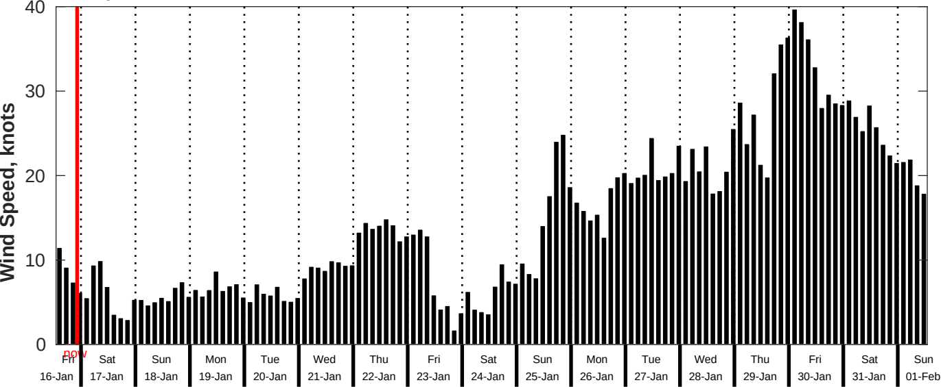
GFS Wind Speed Forecast for NDBC 51209 from 16-Jan-2026 13:00:00 to 01-Feb-2026 13:00:00
