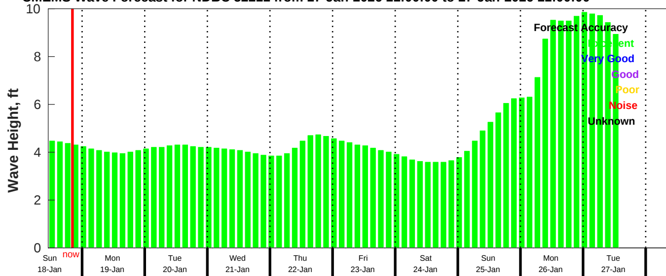
CMEMS Wave Forecast for NDBC 52211 from 17-Jan-2026 11:00:00 to 27-Jan-2026 11:00:00
