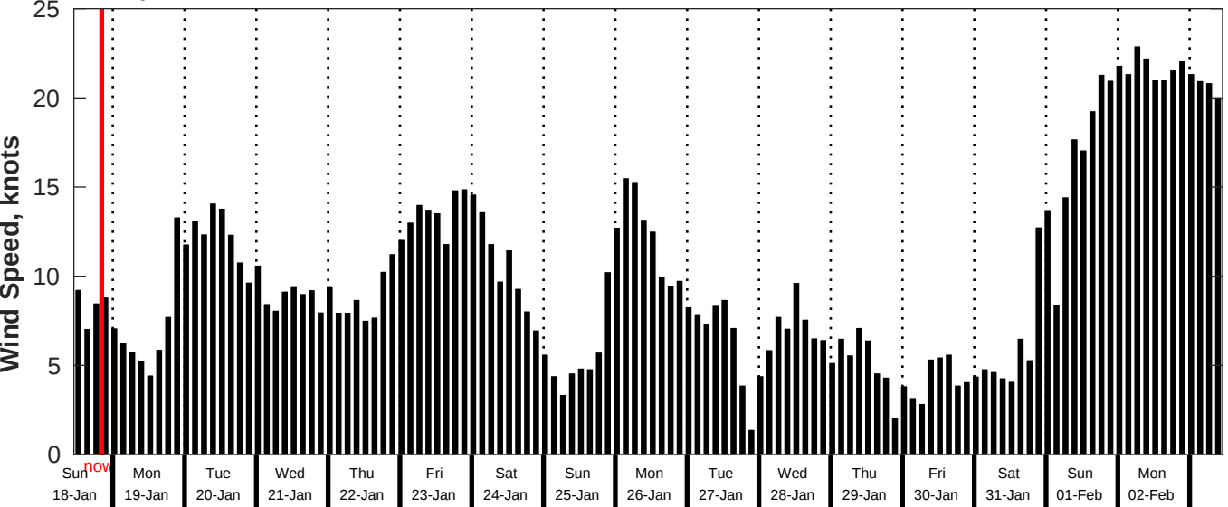
GFS Wind Speed Forecast for NDBC 52211 from 17-Jan-2026 11:00:00 to 02-Feb-2026 11:00:00
