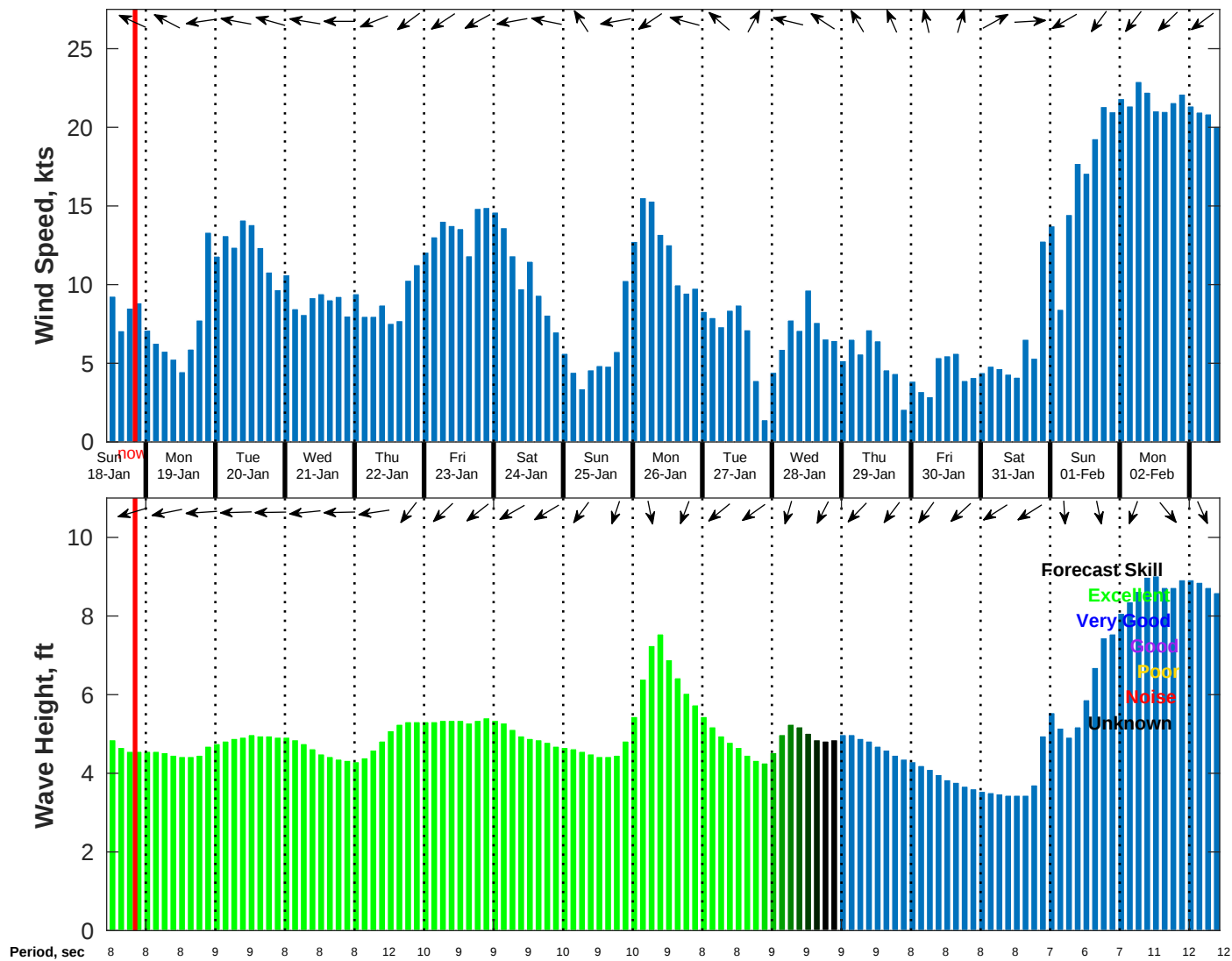
Wind & Wave Forecast for NDBC 52211 from 17-Jan-2026 11:00:00 to 02-Feb-2026 11:00:00
