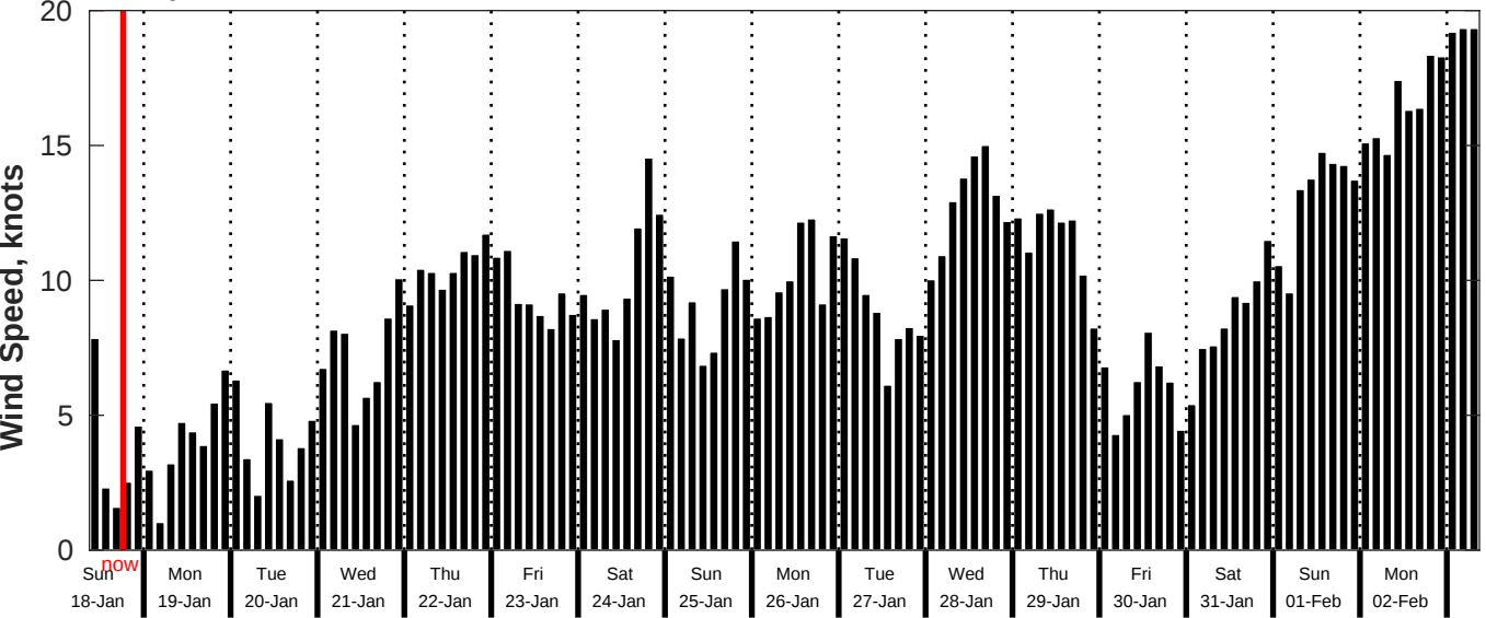
GFS Wind Speed Forecast for NDBC 52212 from 17-Jan-2026 09:00:00 to 02-Feb-2026 09:00:00
