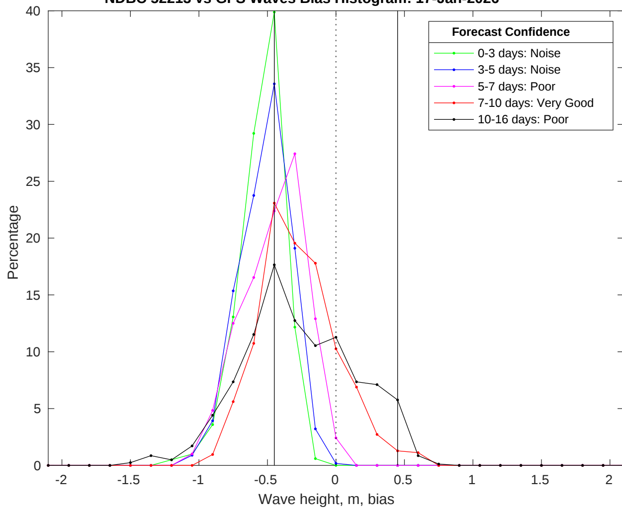
NDBC 52213 vs GFS Waves Bias Histogram: 17-Jan-2026
