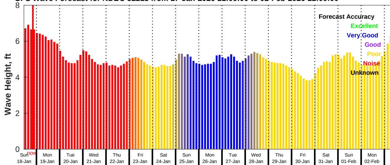
GFS Wave Forecast for NDBC 52213 from 17-Jan-2026 11:00:00 to 02-Feb-2026 11:00:00
