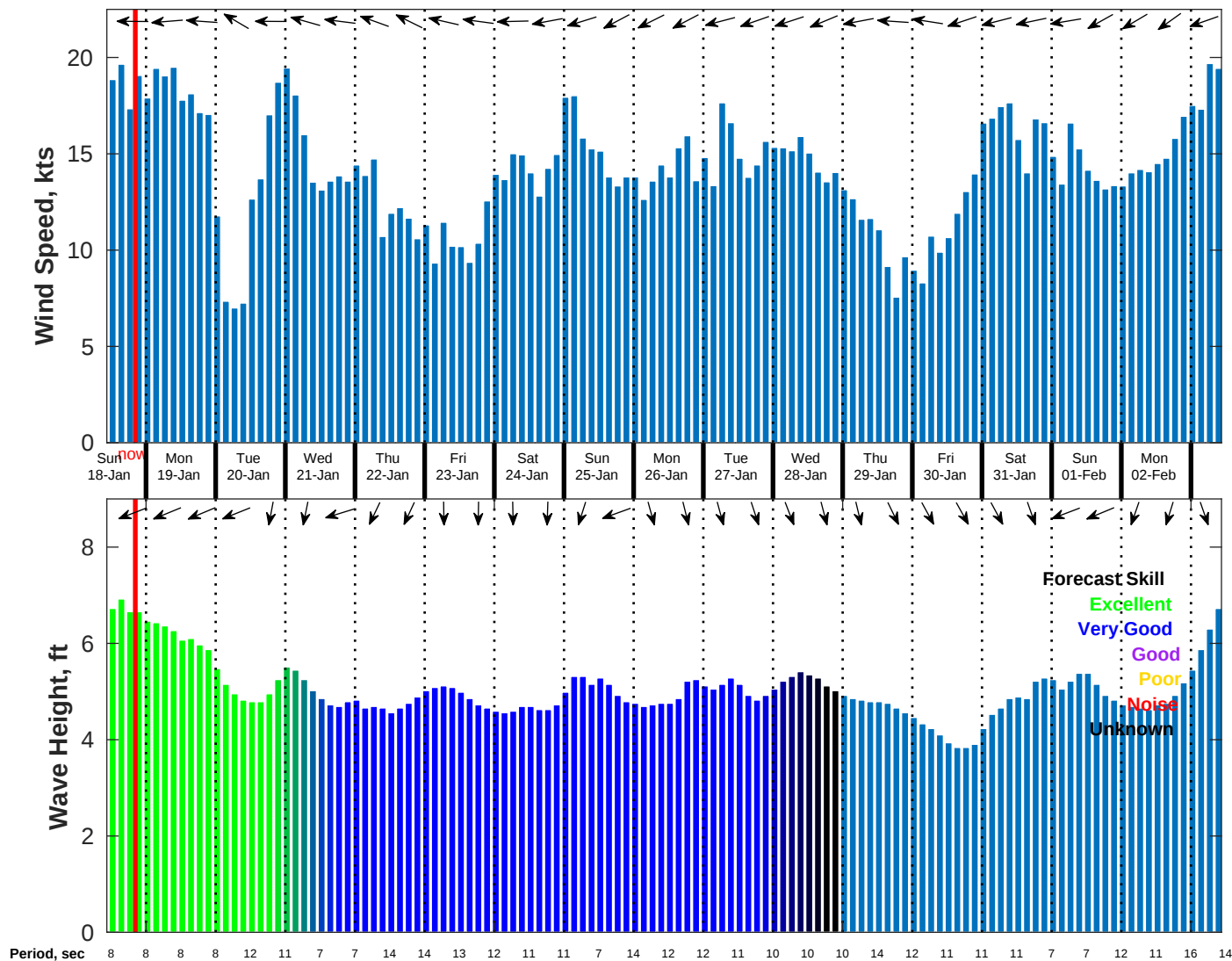
Wind & Wave Forecast for NDBC 52213 from 17-Jan-2026 11:00:00 to 02-Feb-2026 11:00:00
