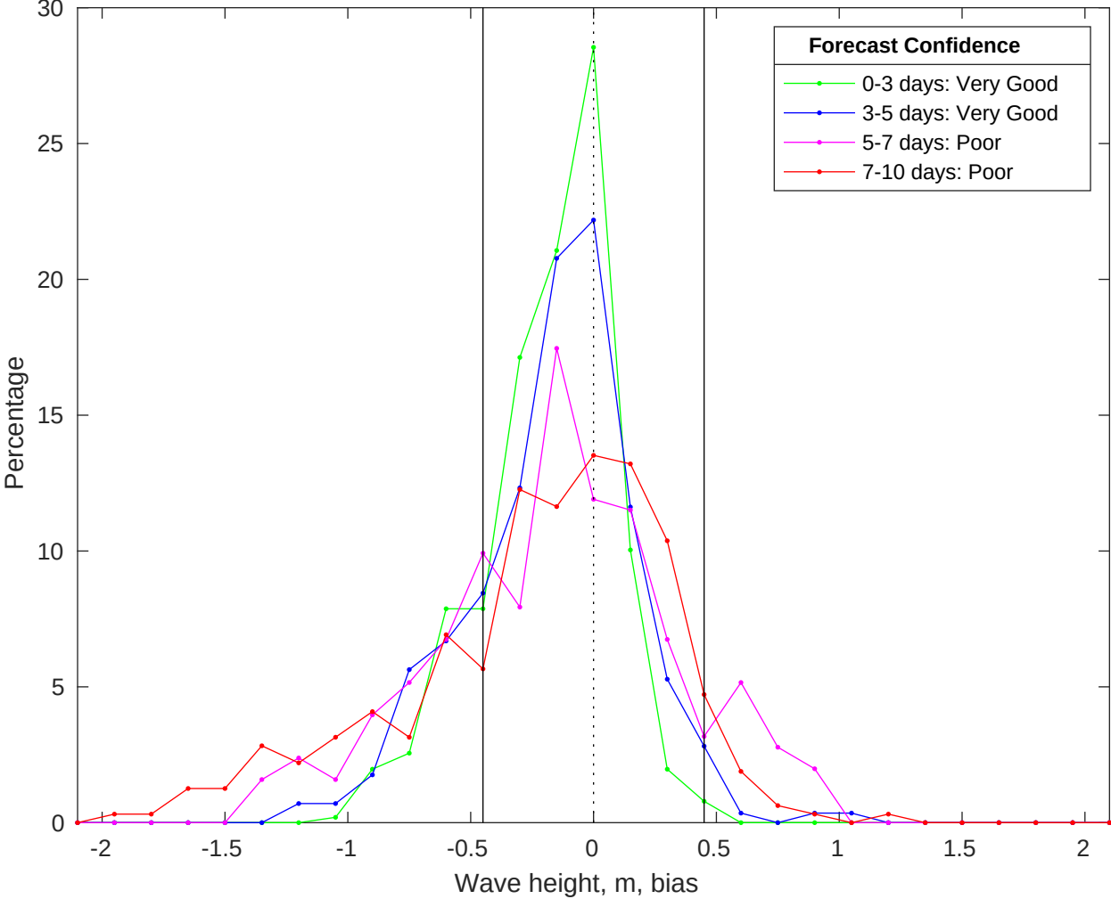
NDBC 41004 vs CMEMS Waves Bias Histogram: 18-Jan-2026
