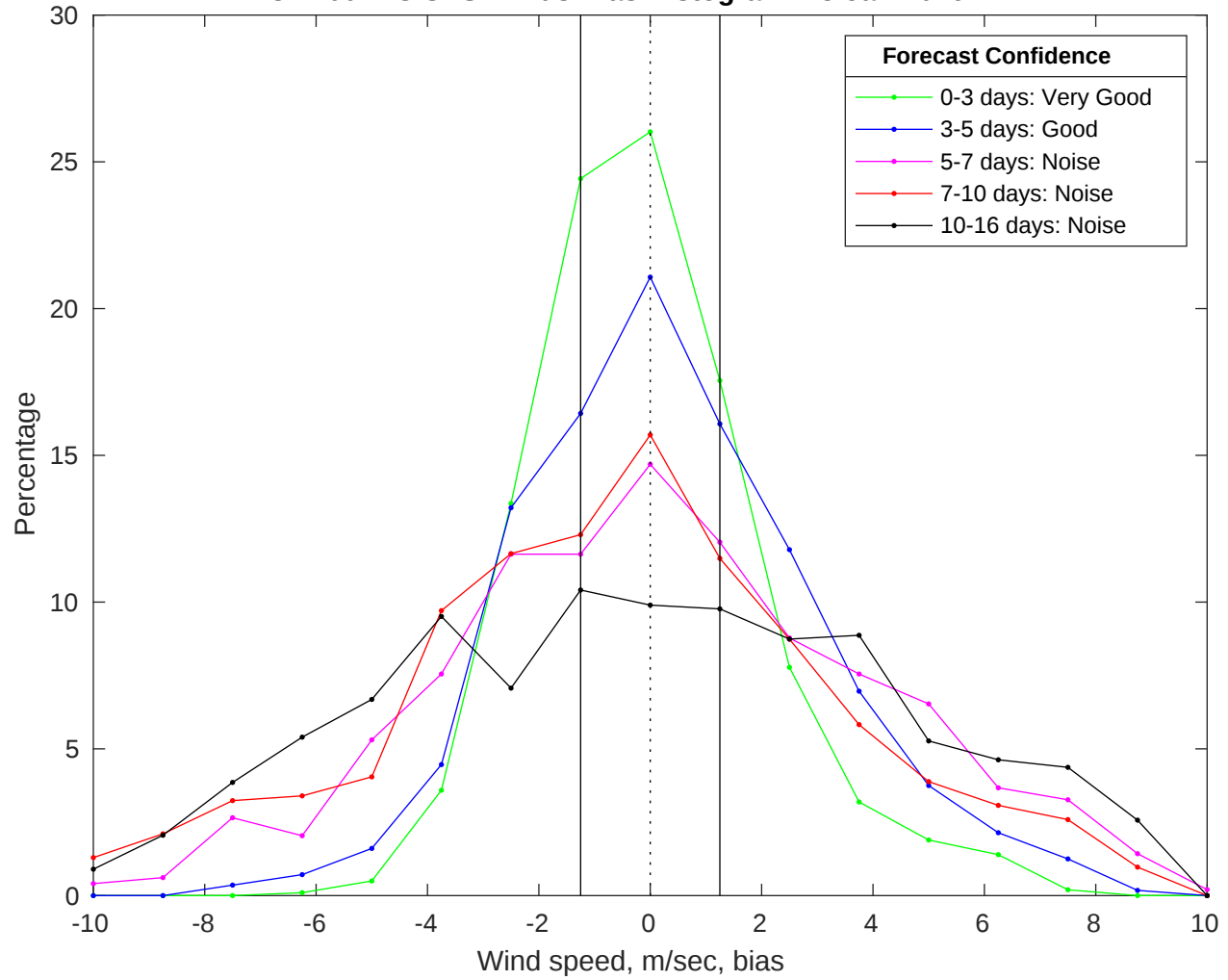
NDBC 41004 vs GFS Winds Bias Histogram: 18-Jan-2026
