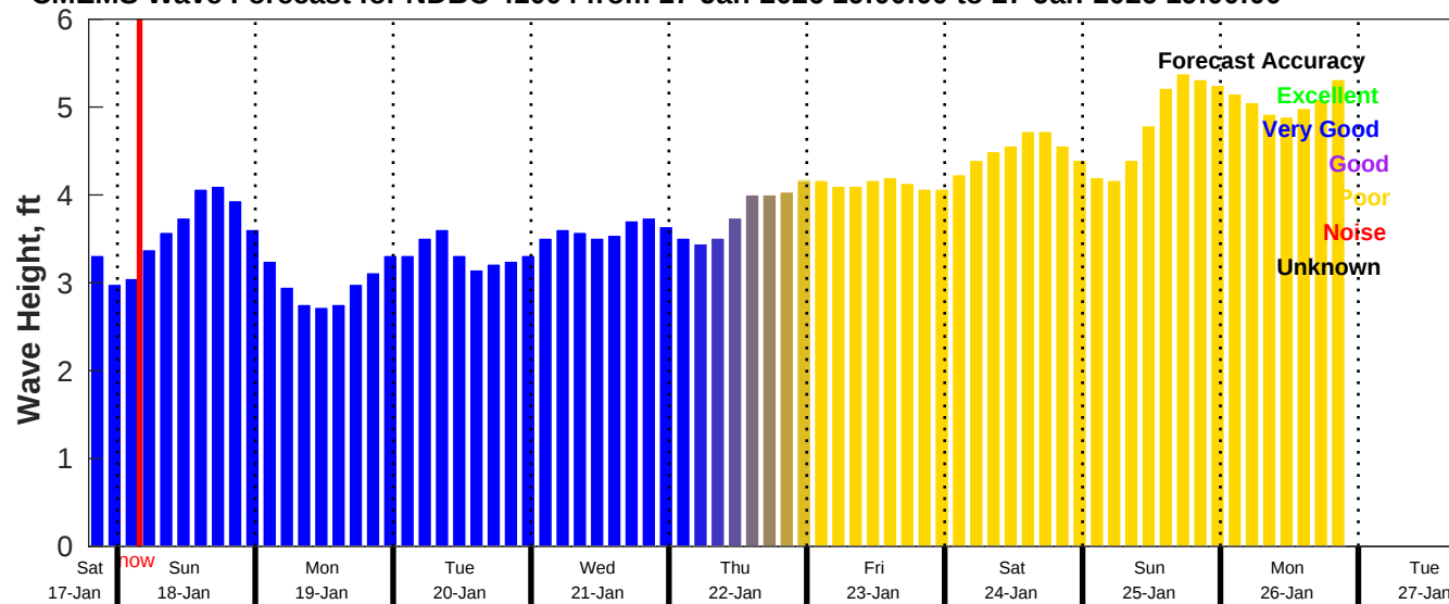
CMEMS Wave Forecast for NDBC 41004 from 17-Jan-2026 19:00:00 to 27-Jan-2026 19:00:00
