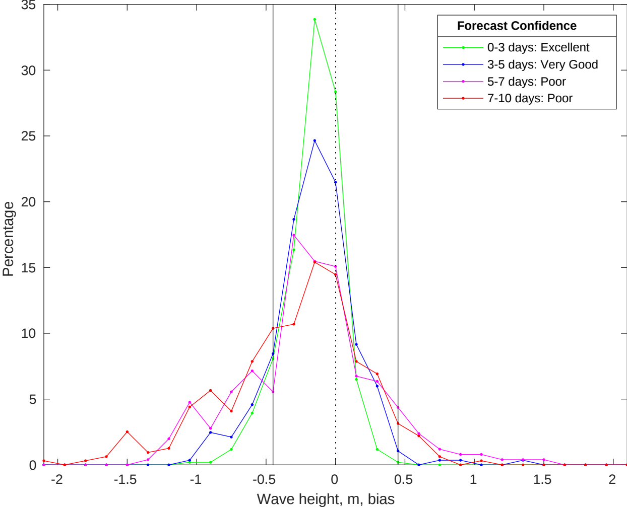
NDBC 41013 vs CMEMS Waves Bias Histogram: 18-Jan-2026
