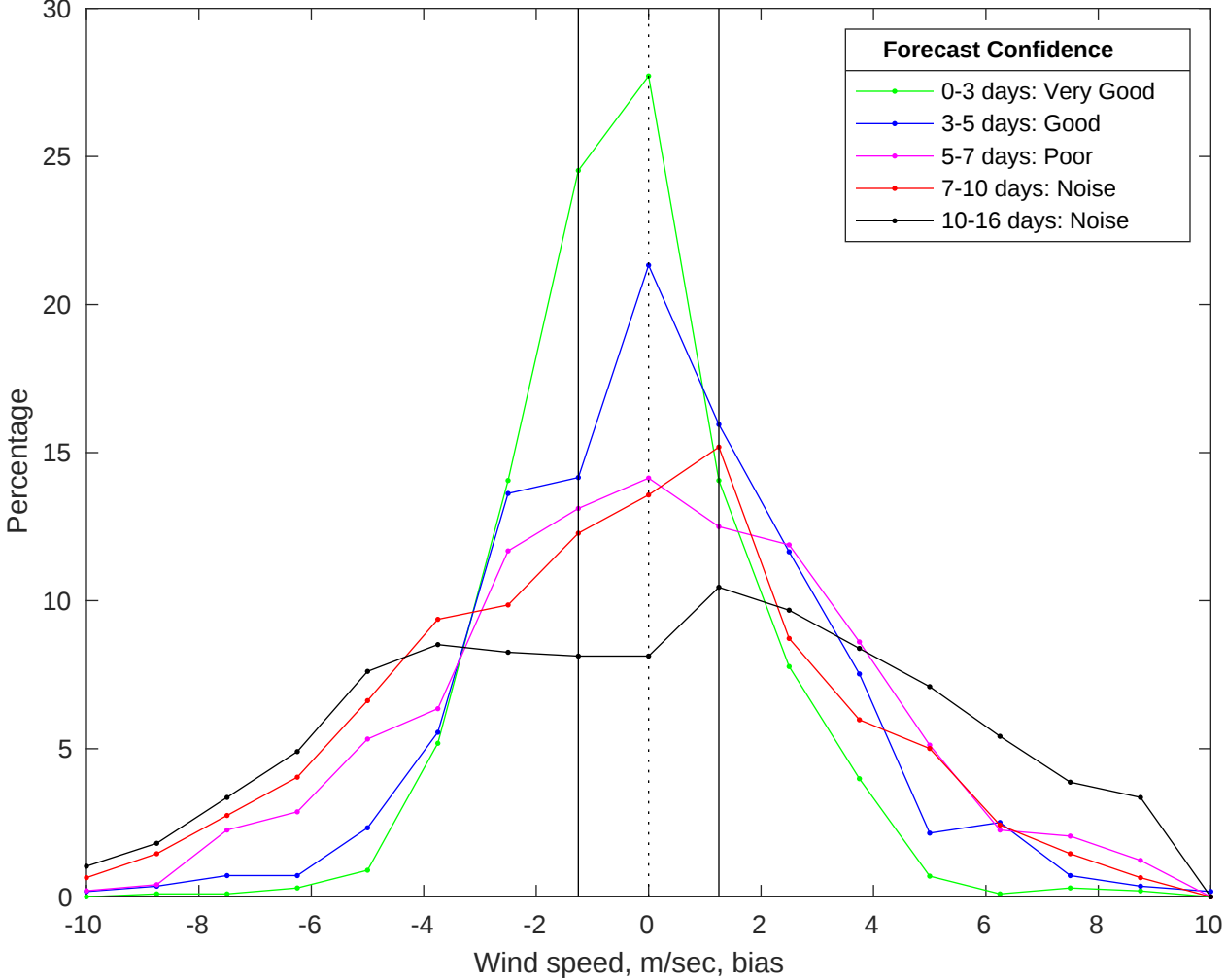
NDBC 41013 vs GFS Winds Bias Histogram: 18-Jan-2026
