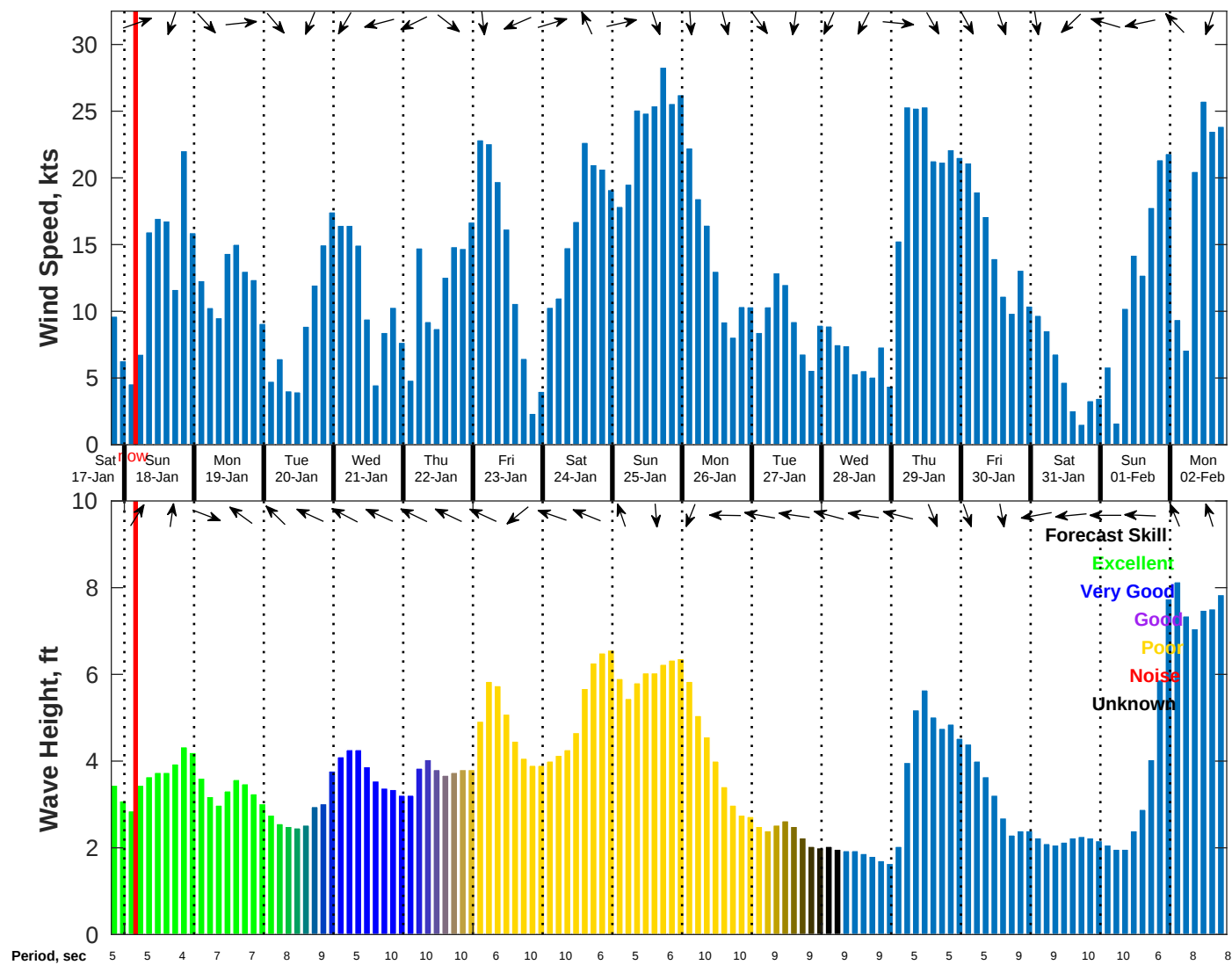
Wind & Wave Forecast for NDBC 41013 from 17-Jan-2026 19:00:00 to 02-Feb-2026 19:00:00
