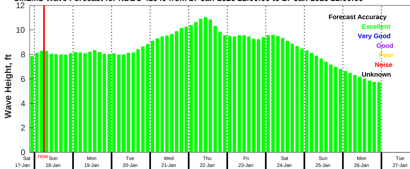
CMEMS Wave Forecast for NDBC 41040 from 17-Jan-2026 21:00:00 to 27-Jan-2026 21:00:00
