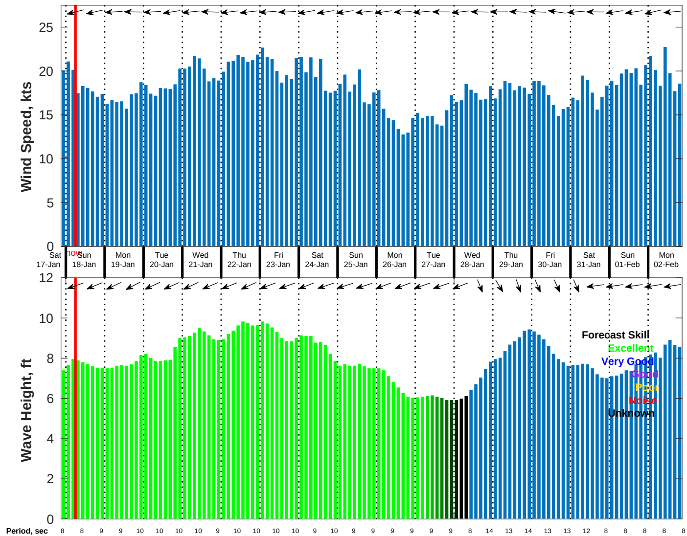
Wind & Wave Forecast for NDBC 41040 from 17-Jan-2026 21:00:00 to 02-Feb-2026 21:00:00
