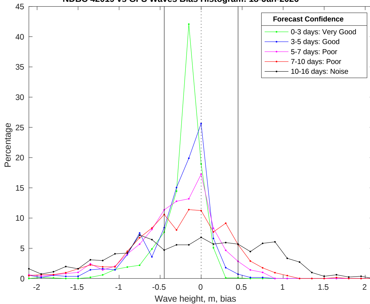
NDBC 42019 vs GFS Waves Bias Histogram: 18-Jan-2026
