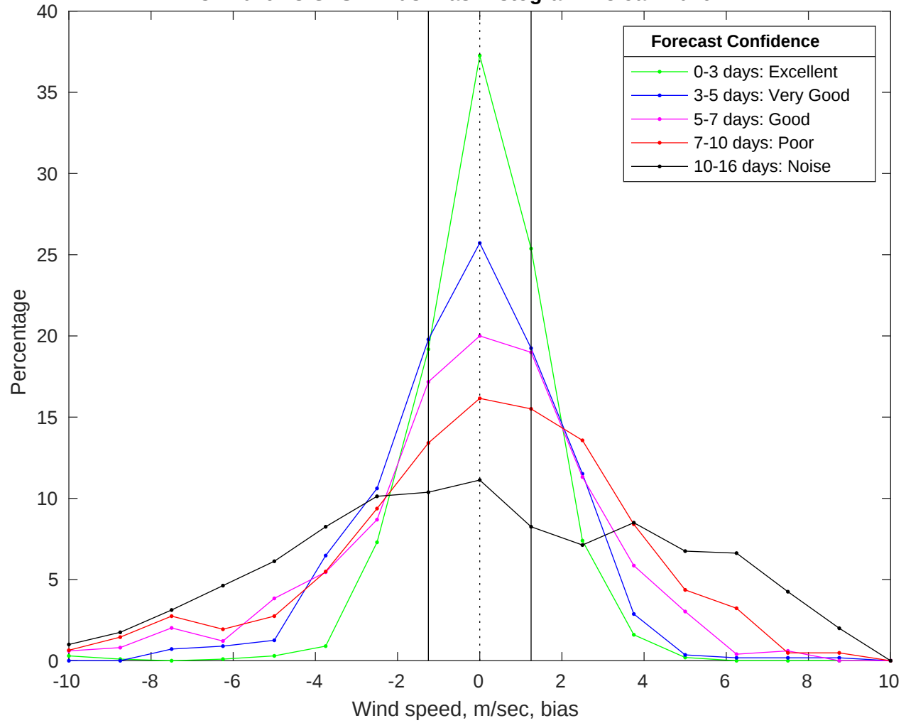
NDBC 42019 vs GFS Winds Bias Histogram: 18-Jan-2026
