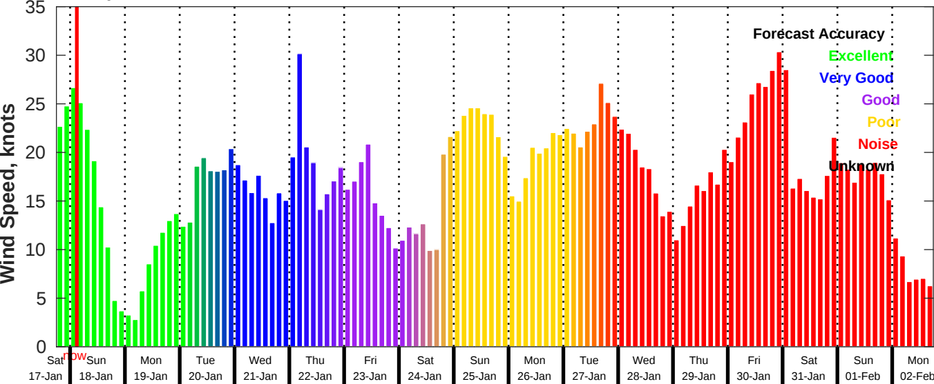
GFS Wind Speed Forecast for NDBC 42019 from 17-Jan-2026 18:00:00 to 02-Feb-2026 18:00:00
